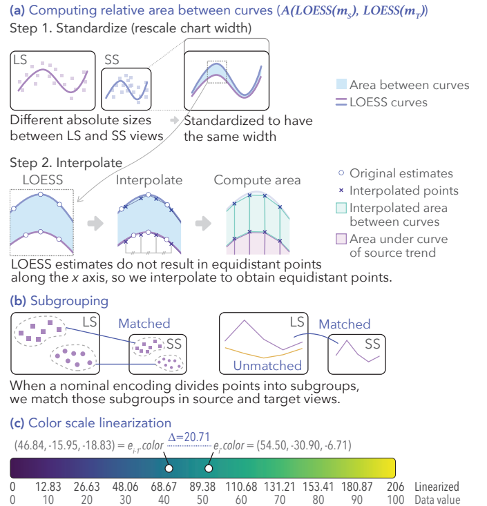
Fig. 7. Components of computing trend loss. (a) Calculating area between curves by standardizing chart size and interpolating break points. (b) Dividing and matching subgroups. (c) Linearizing color scale. LS is large screen, and SS is small screen.
